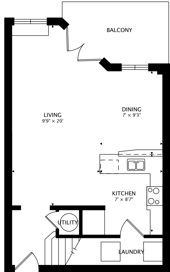
MAIN Main Level
