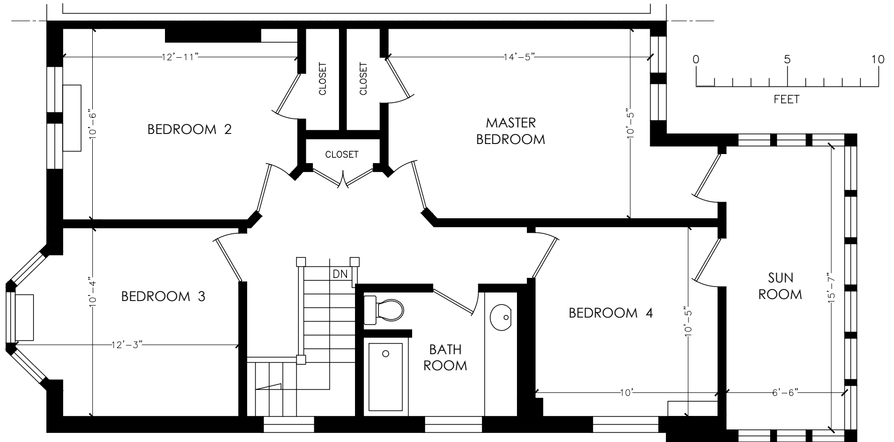
SECOND FLOOR FLOOR AREA 955 SQUARE FEET
